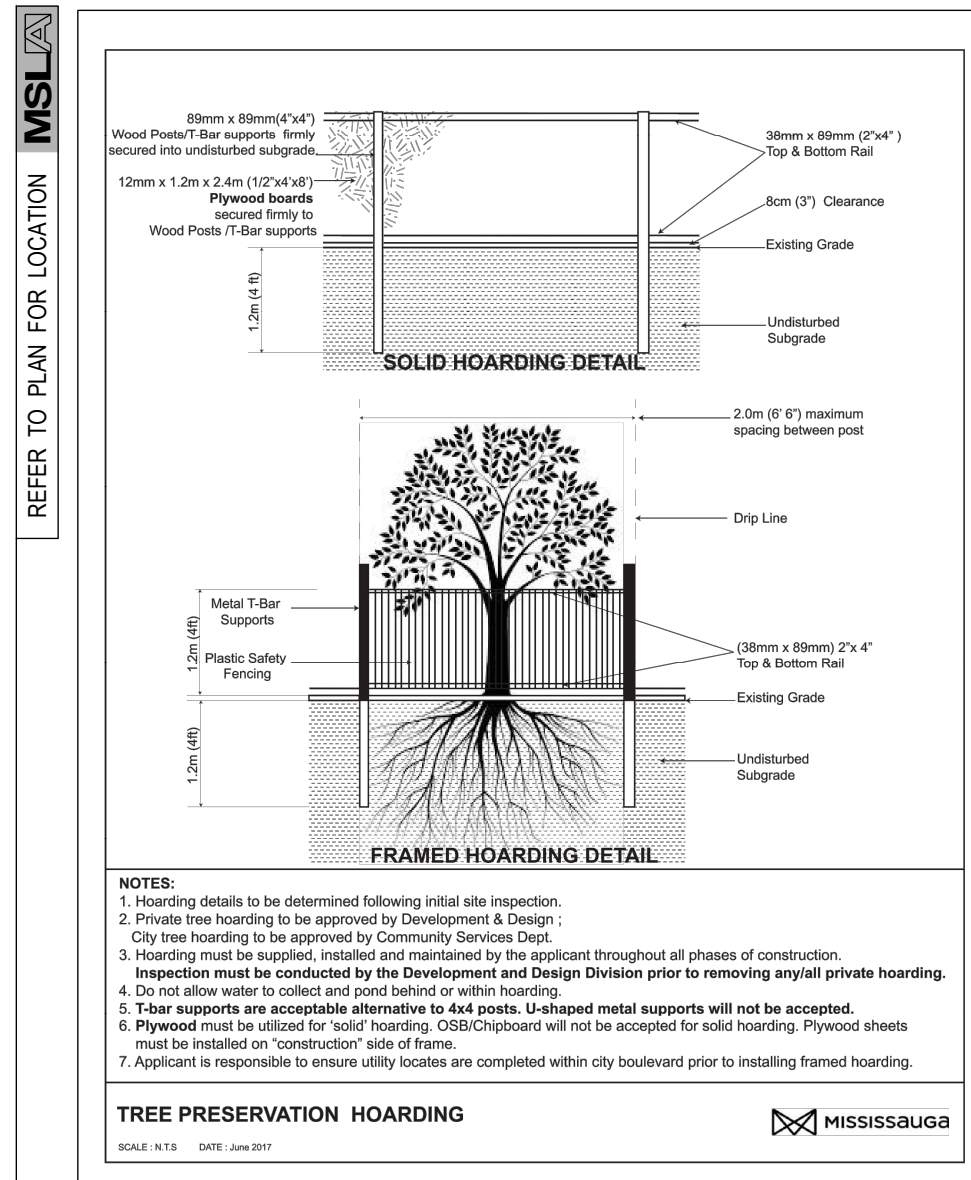
TREE PROTECTION BARRIERS DETAIL TYP.
